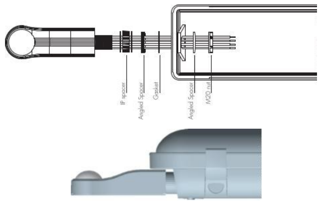
Typical Installation 2
