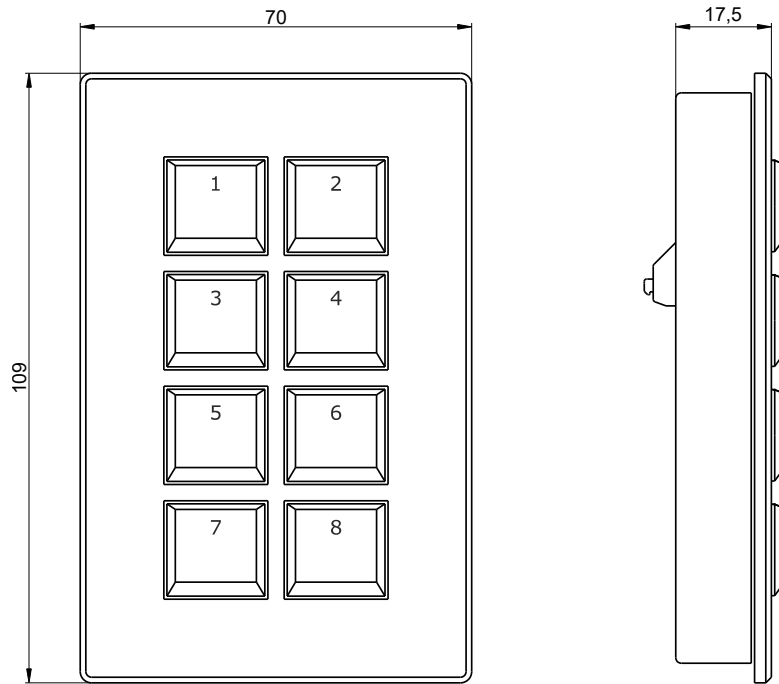
Mounting plate
