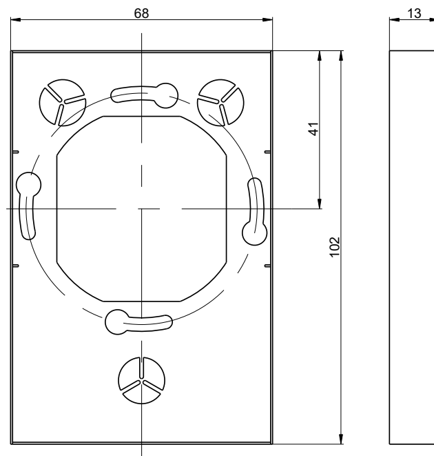
Mounting plate
